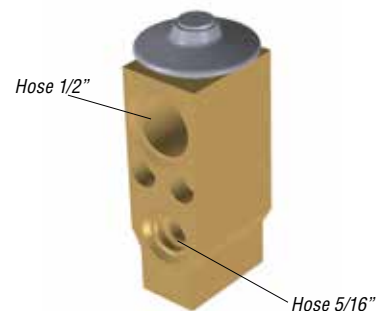
Expansion valve 2.0 TON
